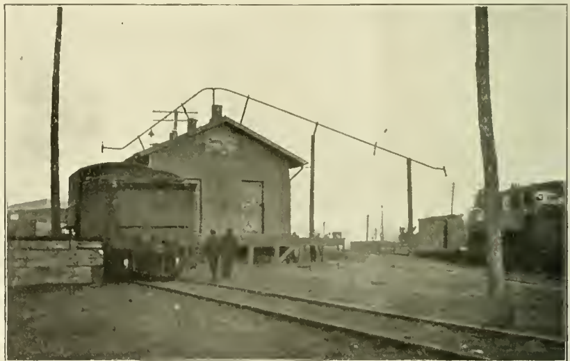
SAND HOUSE AND CONVEYING PIPES AT THE 5TH STREET ROUNDHOUSE OF BALTIMORE & OHIO R.R., PHILADELPHIA, PA.
